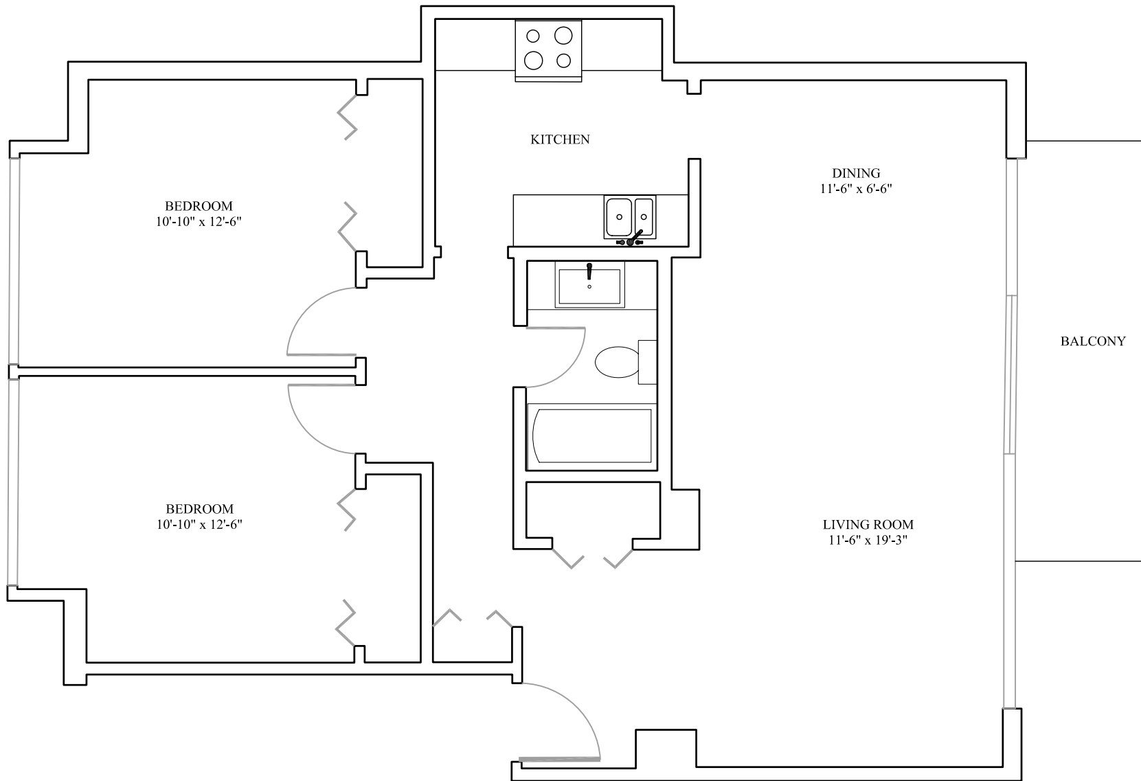
BERN STREET - FLOOR PLAN B TWO BEDROOM 2ND FLOOR - BALCONY / GROUND FLOOR - PATIO
