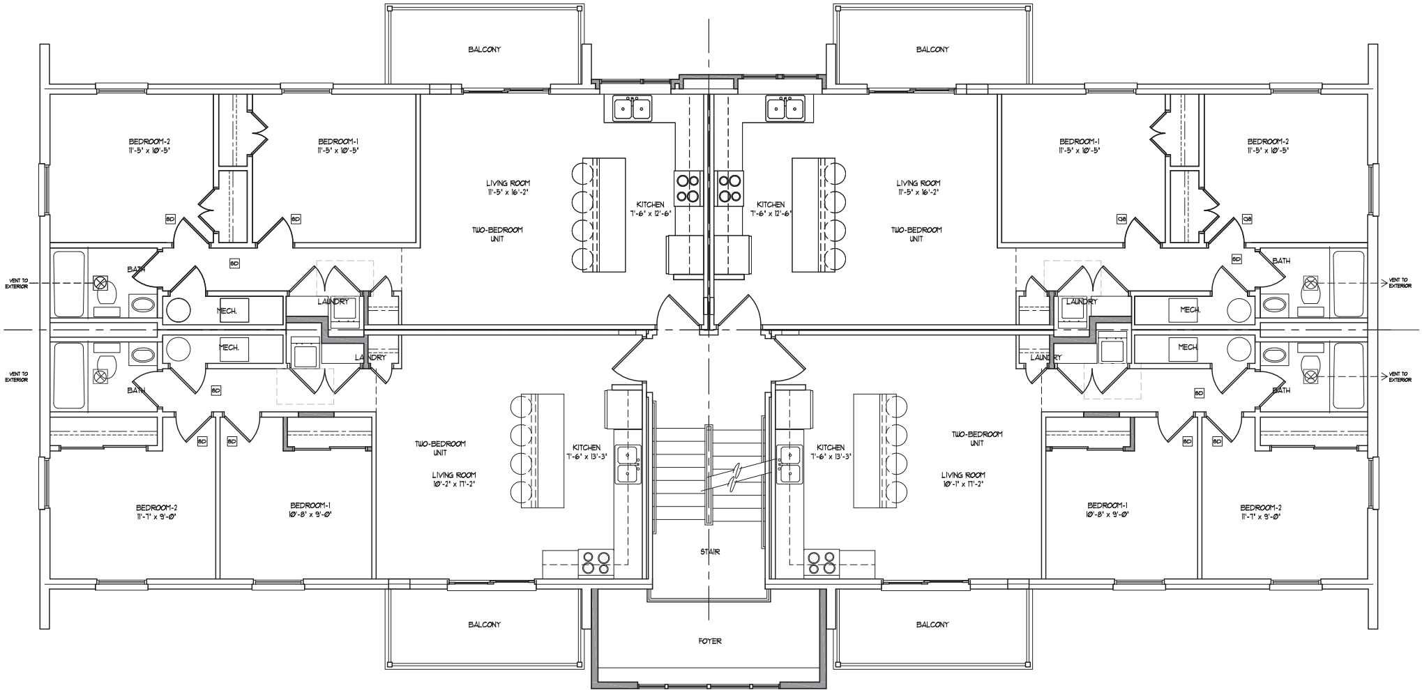
TYP. 2ND & 3RD FLOOR PLANS 1/8" = 1'-0"
