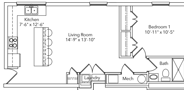
One Bedroom Unit Lower Floor
